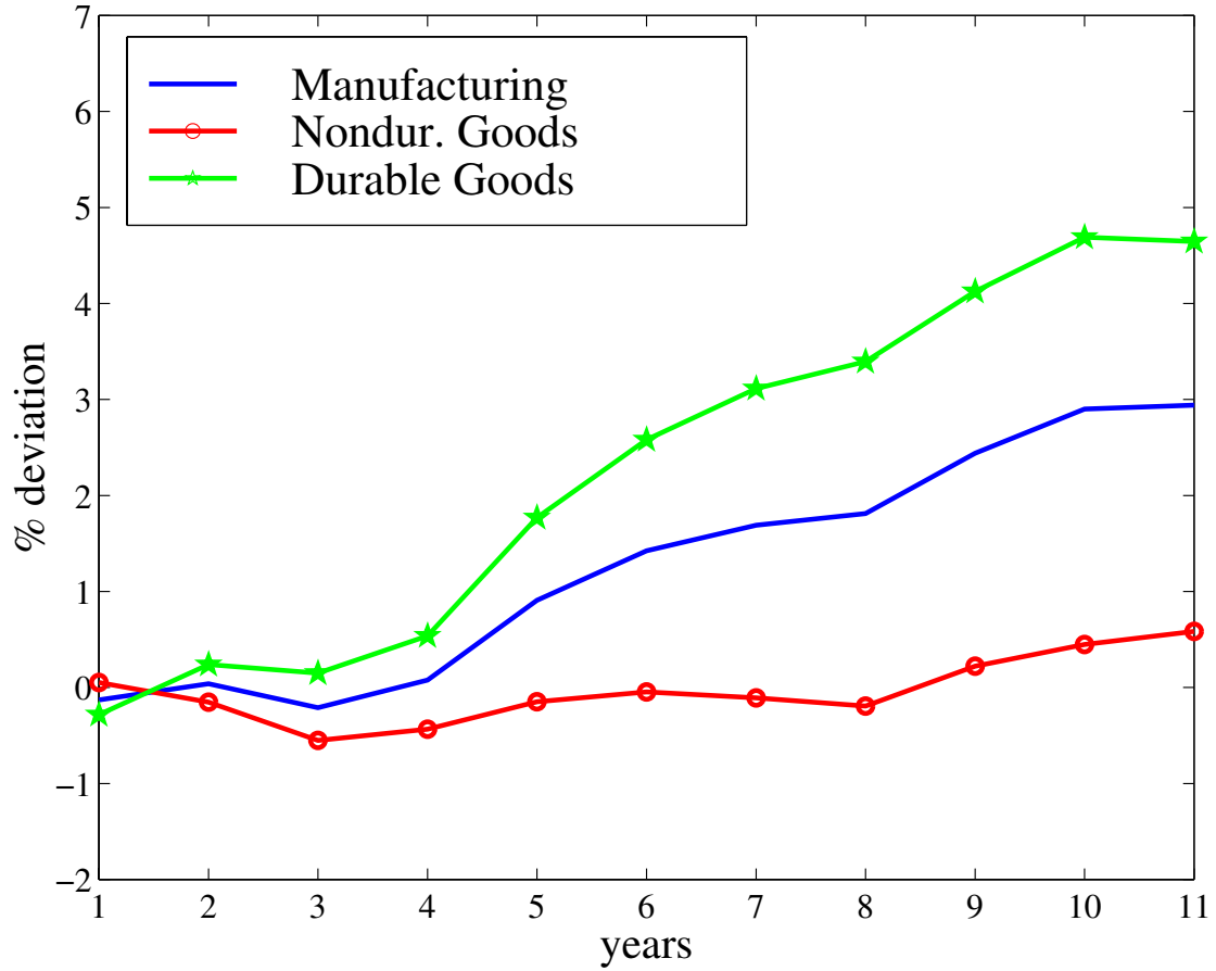
Figure 8: U.S. Sectoral TFP Responses To a Stock market Innovation \epsilon_2
