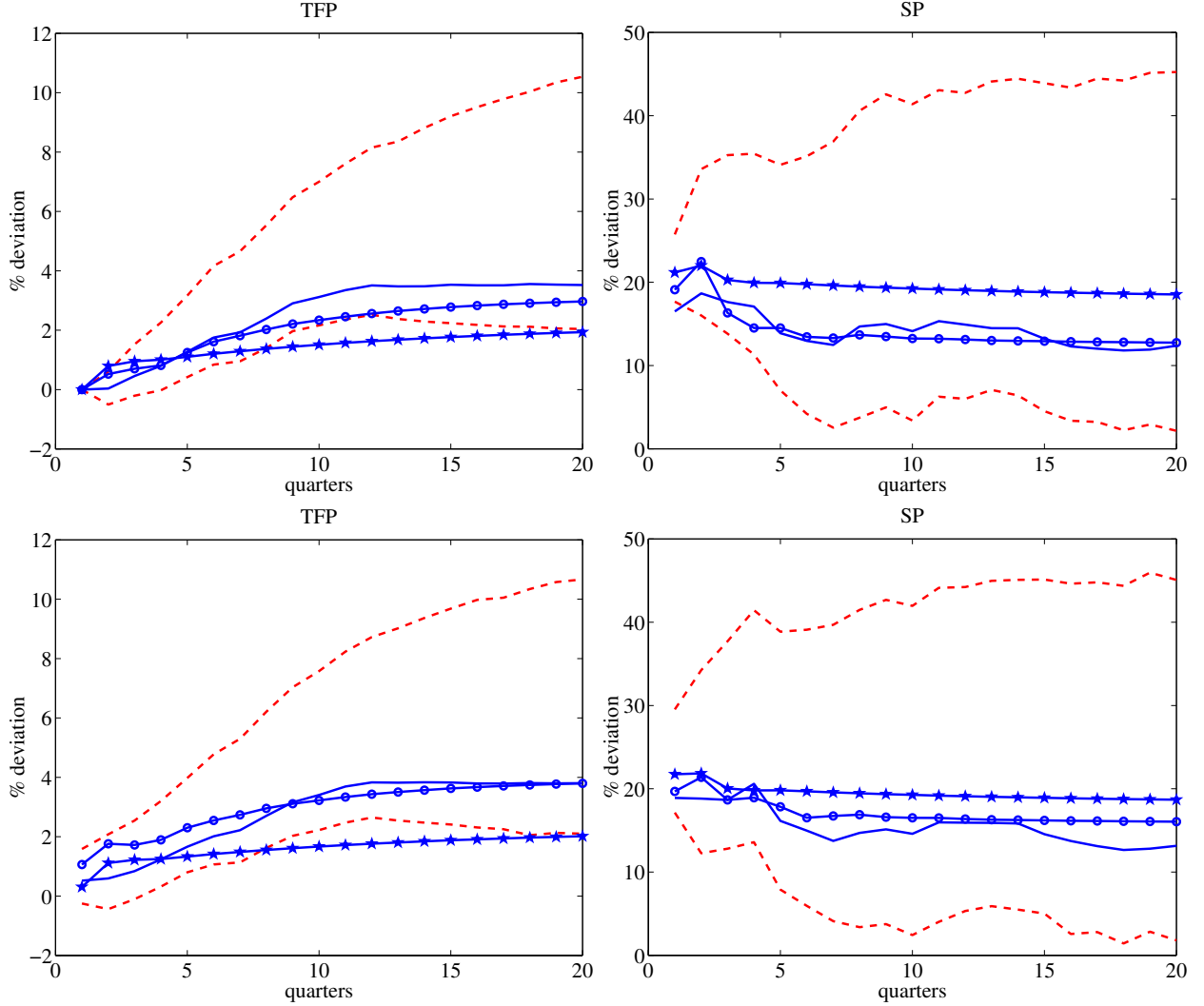
Figure 4: Impulse Responses to Shocks \epsilon_2 and \tilde{\epsilon}_1 in the Japanese ( TFP, SP ) VECM, for different choices of lag length.
