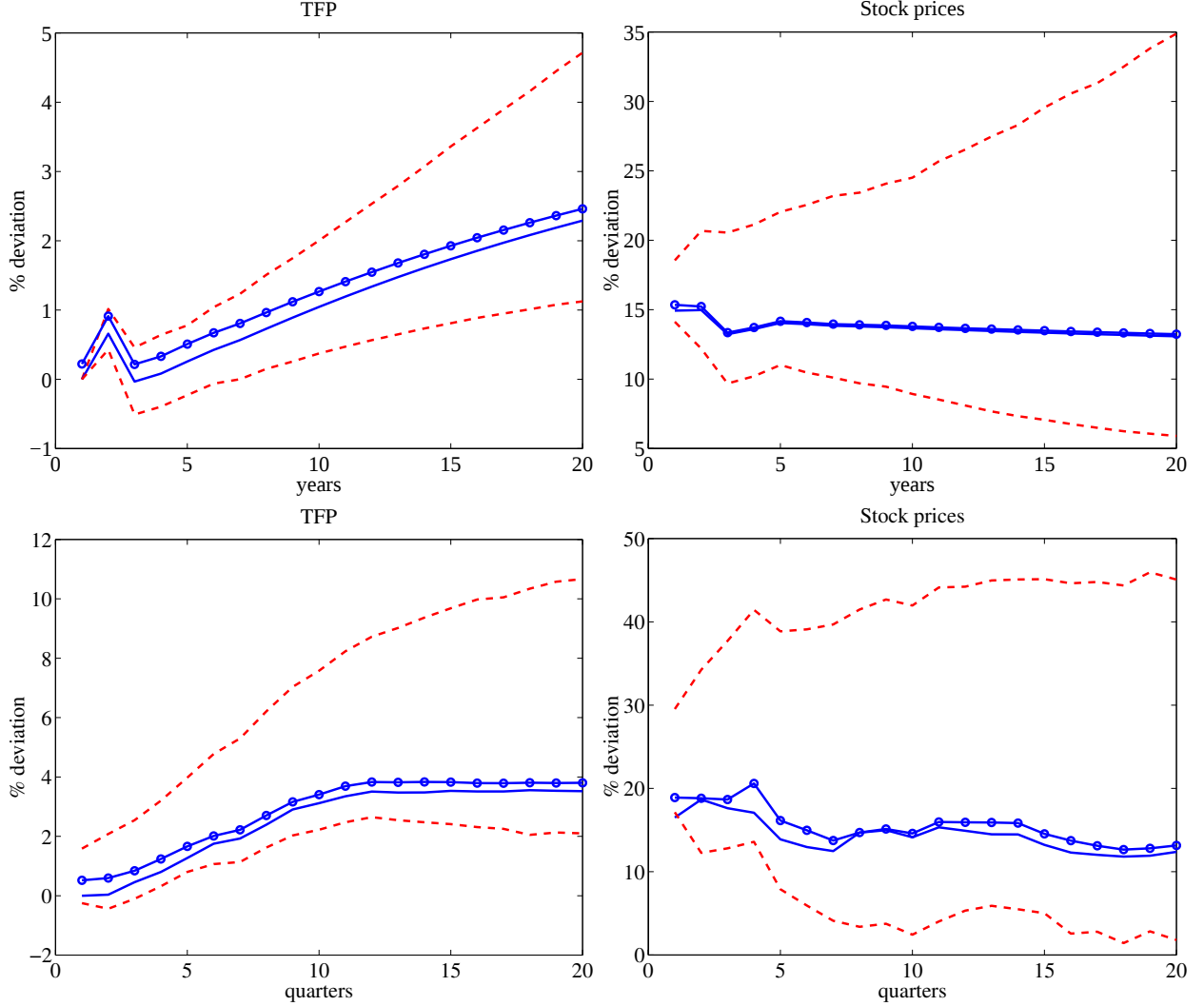
Figure 1: Impulse Responses to Shocks \epsilon_2 and \tilde{\epsilon}_1 in the (TFP, SP) VECM, Using U.S. Data (top line) and Japanese Ones (bottom line)
