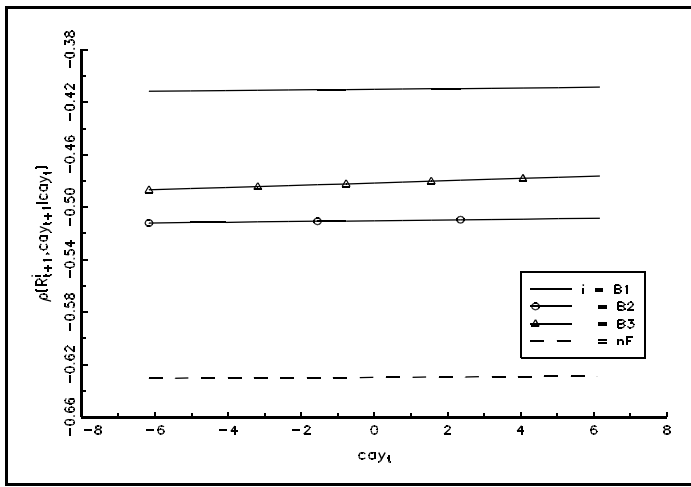
Conditional Correlation
