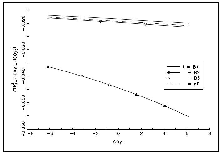
Conditional Covariance
