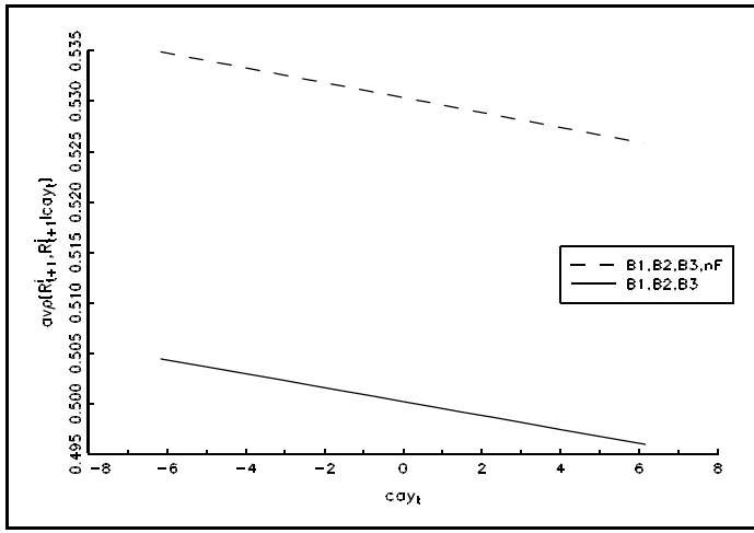
Average Correlation
