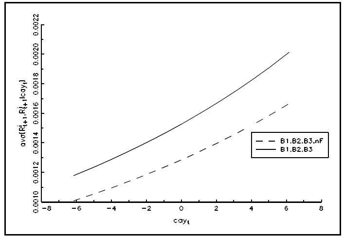
Average Covariance
