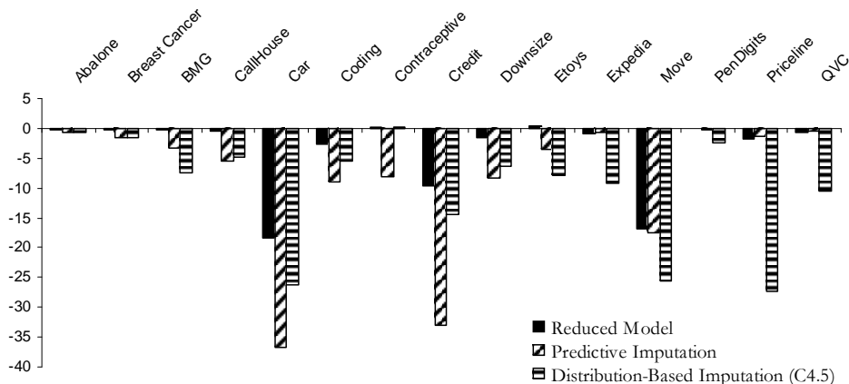
Figure 6: Relative differences in accuracy for bagged decision trees between each missing value treatment and the complete setting where all feature values are known.
