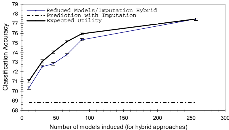
Figure 11: Performance of Utility-Based Hybrid of Reduced Models and Imputation
