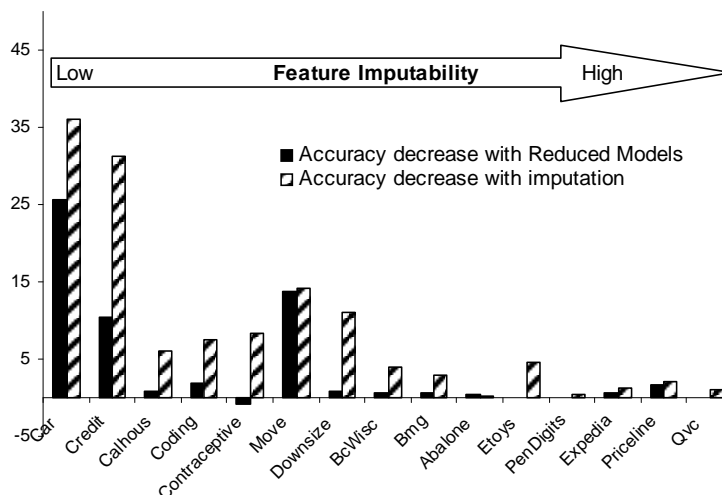
Figure 5: Decrease in accuracy for reduced-feature modeling and value imputation. Domains are ordered left-to-right by increasing feature imputability. Reduced modeling is much more robust to moderate levels of feature imputability.
