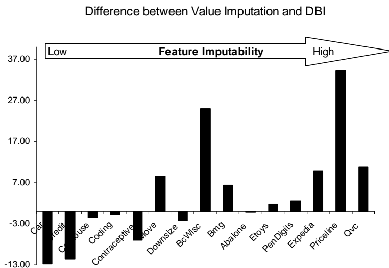
Figure 4: Difference between the relative performances of PVI and DBI. Domains are ordered left-to-right by increasing feature imputability. PVI is better for higher feature imputability, and DBI is better for lower feature imputability.
