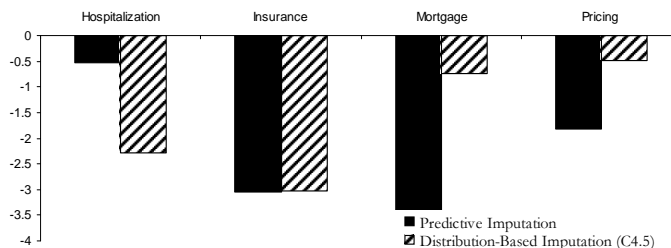
Figure 9: Relative percentage-point differences in predictive accuracy obtained with distribution-based imputation and predictive value imputation treatments compared to that obtained with Reduced Models
