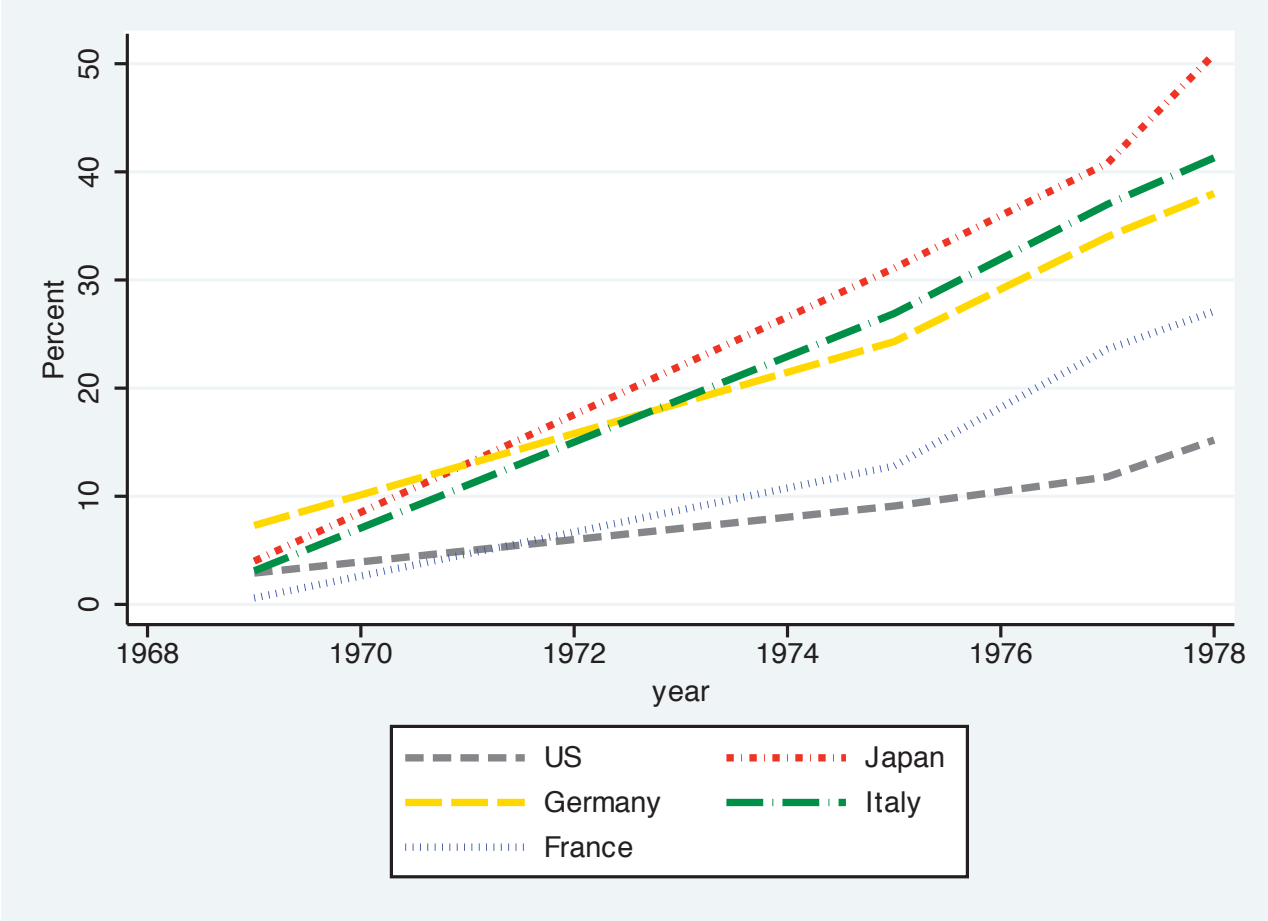
Figure 7: Fraction of Steel Made Using Continuous Casting Process
