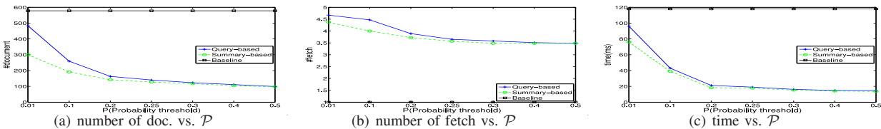
Fig. 1. Varying \mathcal{P}
