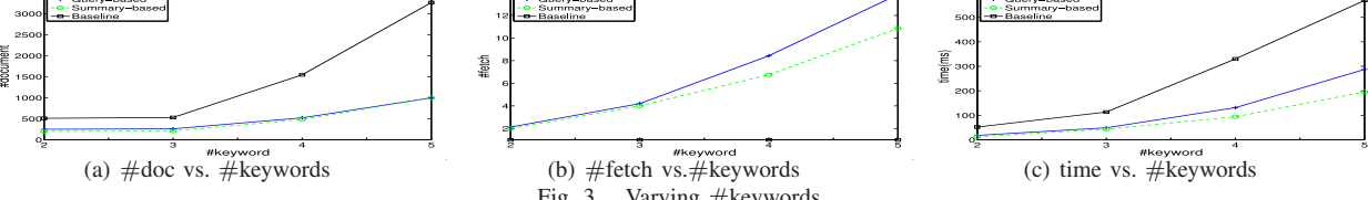
Fig. 3. Varying #keywords
