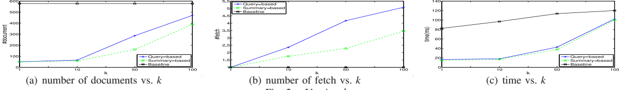
Fig. 2. Varying k
