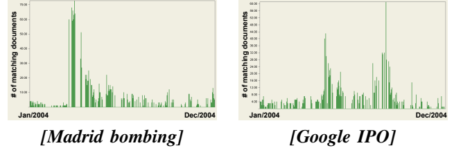
Fig. 1. Histograms for queries [Madrid bombing] and [Google IPO] , showing the number of documents with all query words for each day from January to December 2004 in a news archive.
