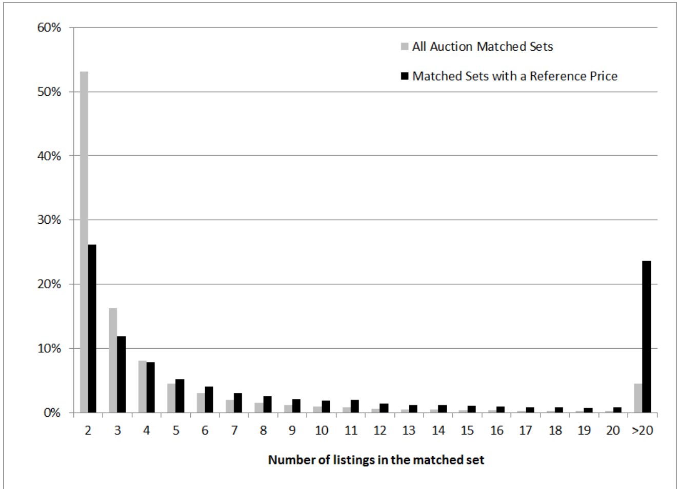
Figure 2: Number of listings in each matched set
