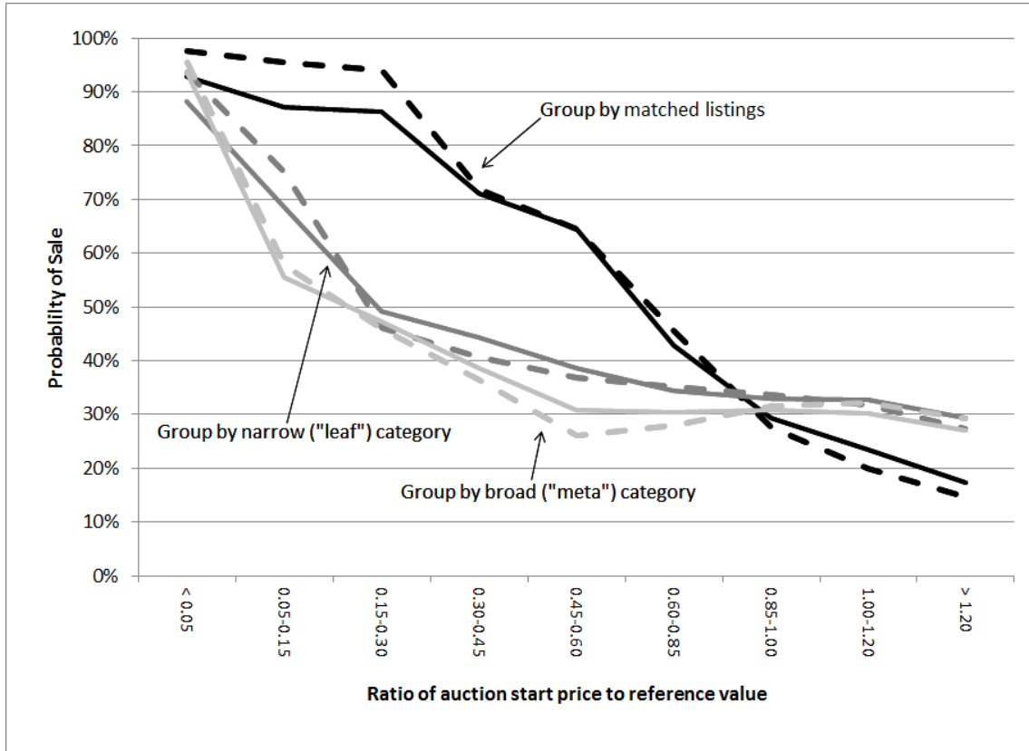
Figure 7: Matched listings approach versus cross-item observational data
