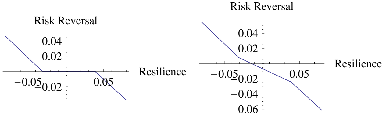
Figure 2: Risk-Reversal vs Resilience. Units are annualized. The figure plots the Risk-Reversal (28) vs the resilience \hat{H}_B , assuming the country A is at the steady state, \hat{H}_A = 0 . The Figure illustrates that when country B is riskier, its risk-reversal is higher. The left panel corresponds to no noise, and the right panel corresponds to a noise \nu = 0.5 .
