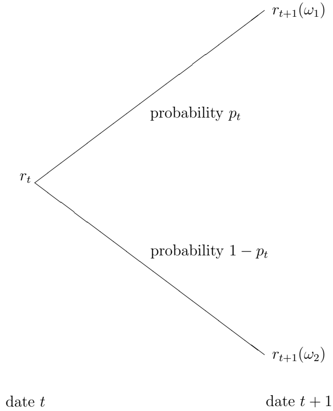
Figure 1: A representation of the recursive constraint game in discrete time using a binomial specification. The entropy level r_t is given as of date t , and the minimizing player chooses a distorted state probability and state-dependent continuation entropy levels r_{t+1}(\omega) . The current period r_t limits the probability distortion and next period continuation entropies. Continuation entropies are discounted, averaged using the distorted probabilities, and added to the relative entropy from the current period.
