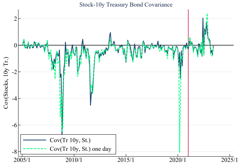
Figure A1: Stock-bond Covariance. Calculation with three daily returns in blue, calculation with single daily returns in dashed neon green. Monthly data from 2005 to 2022. Vertical line indicates 1/2021.
