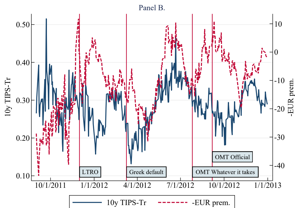
Figure 6D: TIPS-Treasury Premium and Relative Treasury Convenience Yield of German Bunds. Vertical lines correspond to event days described in Table 11A, Panel A.
