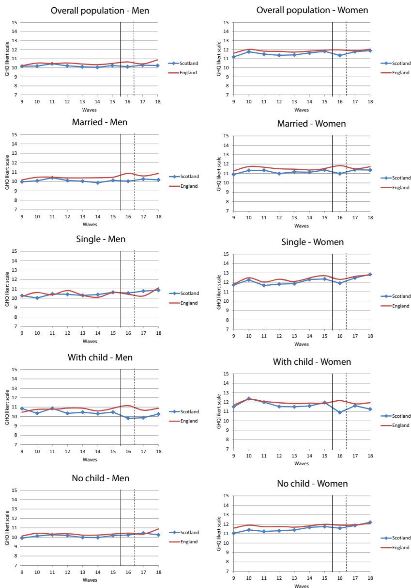
Figure 1. GHQ trends in Scotland and England (after kernel matching).
