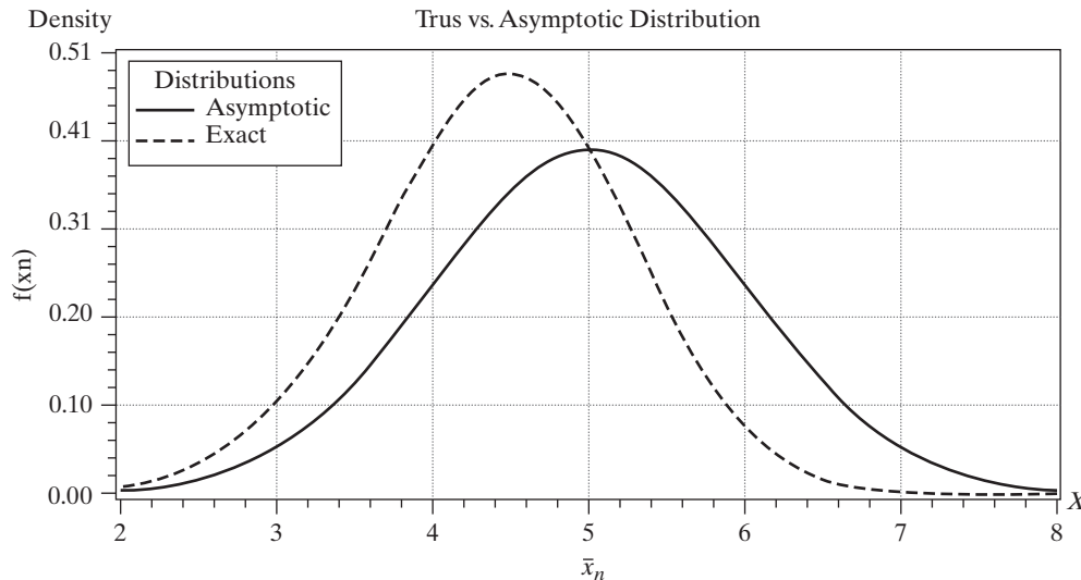
FIGURE D.4 True Versus Asymptotic Distribution.
