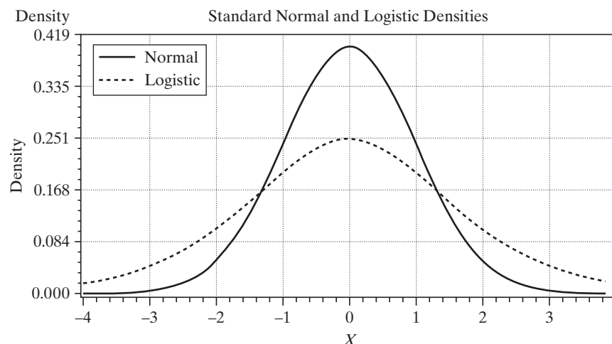
FIGURE B.5 Normal and Logistic Densities.
